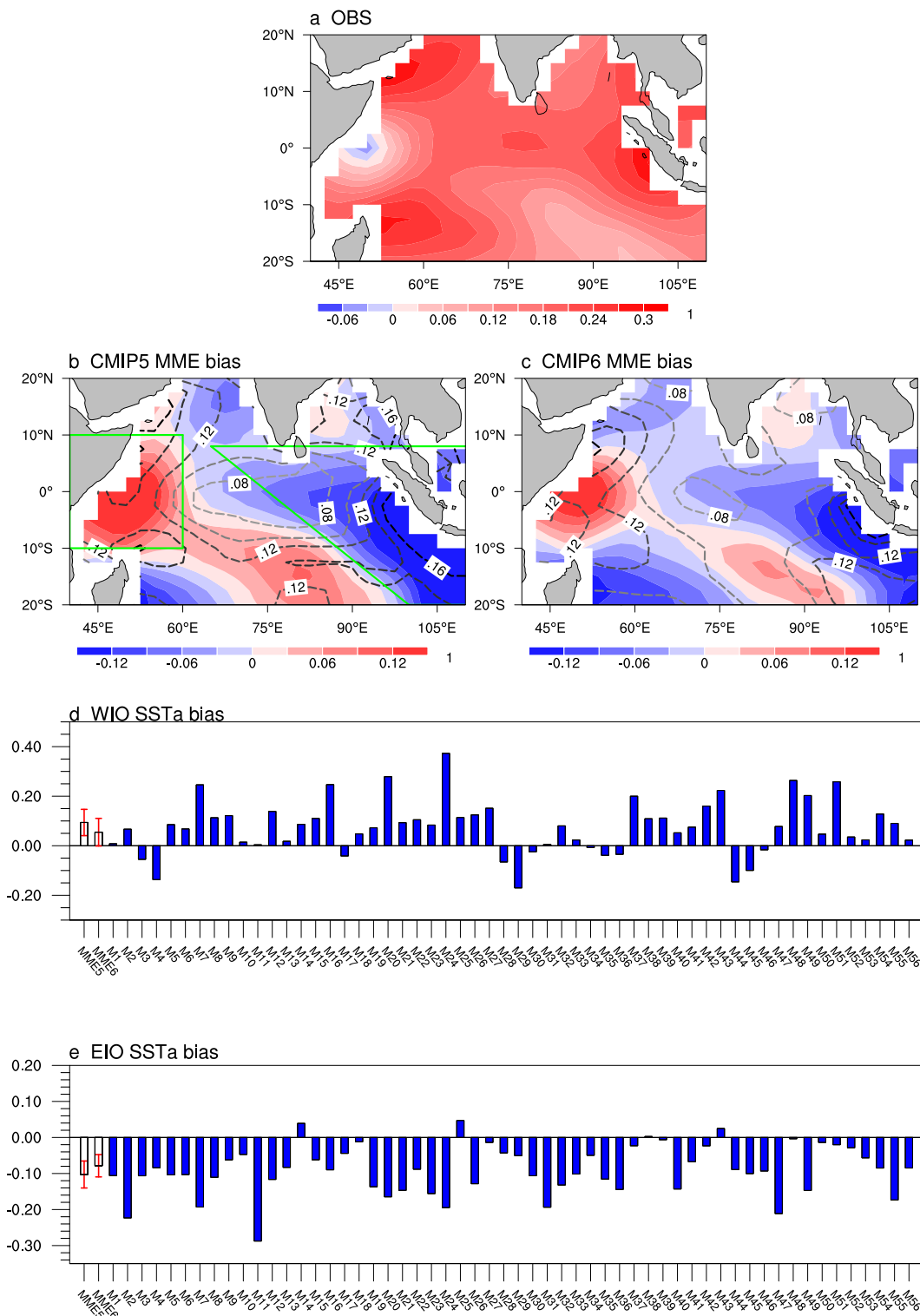
FIG. 1. IOBM patterns during ENSO decay summers [JJA(1)] in (a) observations and associated model biases in (b) the CMIP5 MME and (c) the CMIP6 MME. Shading in (a)–(c) represents SST anomalies regressed onto the D(0)JF(1) Niño-3.4 index, and contours in (b) and (c) indicate intermodel standard deviations. The green box and trapezoid mark the WIO and EIO regions used for area-mean calculations, respectively. (d),(e) The corresponding area-mean ENSO-related SST anomaly biases in the WIO and EIO for the CMIP5 and CMIP6 MMEs, respectively, along with results from individual models.
