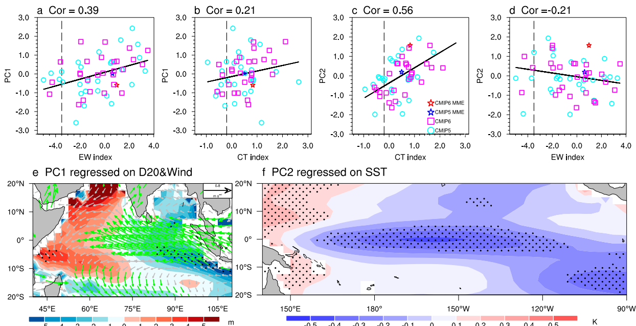
FIG. 3. Intermodel relationships between (a) PC1 and the EW index and (b) PC1 and the CT index. (c),(d) Intermodel correlations between PC2 and the CT index and PC2 and the EW index, respectively. Linear correlation coefficients are shown in the top-left corner of each panel, with solid black lines indicating the linear regression fits. Dashed lines along the horizontal axes represent the observed present-day values of (a),(d) the EW index and (b),(c) the CT index, both multiplied by -1 . (e) Intermodel regression of climatological SON 925-hPa winds and DJF thermocline depth (D20) over the Indian Ocean onto standardized PC1 across 56 CMIP5 and CMIP6 models. (f) Intermodel regression of DJF climatological SST over the Pacific onto standardized PC2. Stippling in (e) and (f) and green wind vectors in (e) indicate regions where the regression is statistically significant at the 90% confidence level based on the Student's t test.
