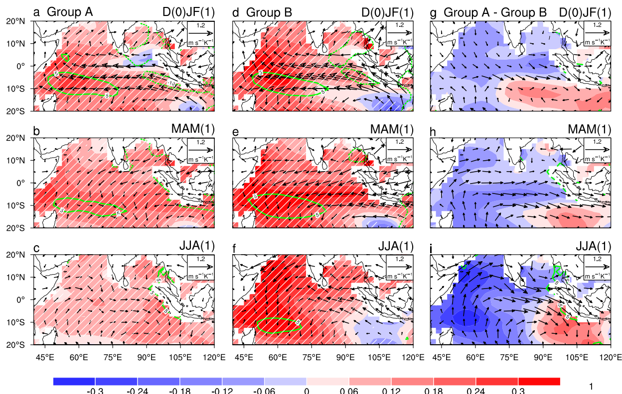
FIG. 5. ENSO-related anomalies for (a)–(c) group A, (d)–(f) group B, and (g)–(i) the MME difference between the two groups. Anomalies of SST (shading, nondimensional), thermocline depth (contours; \text{m K}^{-1} ), and 925-hPa winds (vectors; \text{m s}^{-1} \text{K}^{-1} ) from D(0)JF(1) to JJA(1). Stippled regions in (a)–(f) indicate where the sign of the MME agrees in more than 68% of models. The MME difference in (g)–(i) represents a contrast between ensemble means rather than a statistically tested difference.
