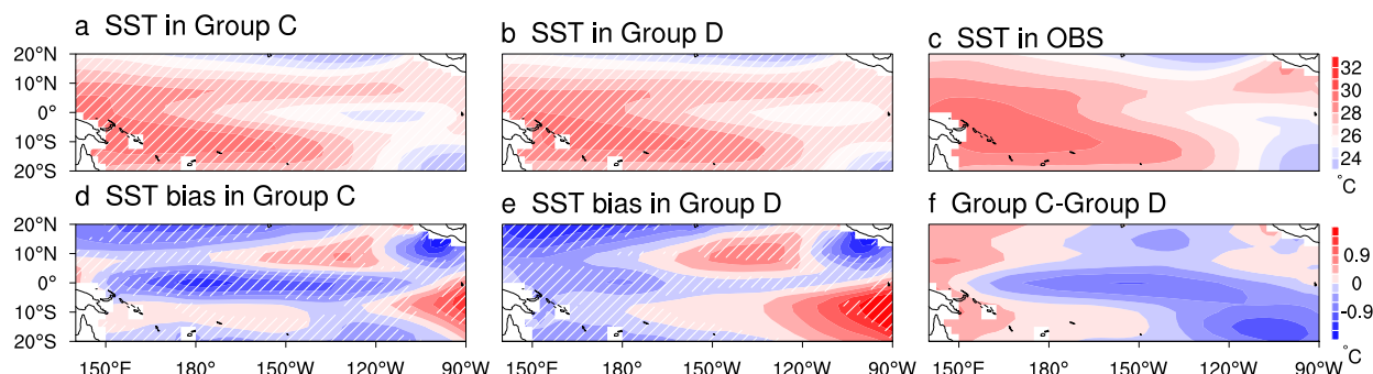
FIG. 6. Climatological SST (shading; ^{\circ}\text{C} ) during winter (DJF) for (a) group C, (b) group D, and (c) observations and MME biases of climatological SST for (d) group C, (e) group D, and (f) the difference between the two groups. Stippled regions in (a), (b), (d), and (e) indicate where the sign of the MME agrees in more than 68% of models. The MME difference in (f) represents a contrast between ensemble means rather than a statistically tested difference.
