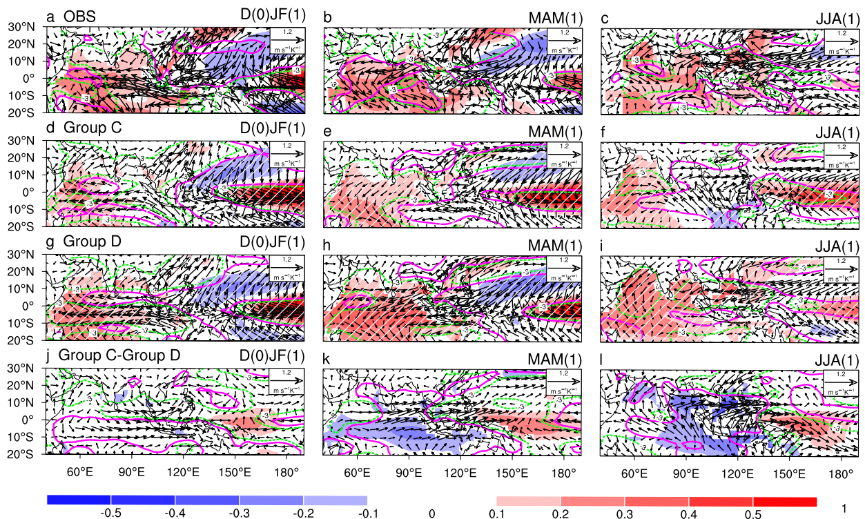
FIG. 7. ENSO-related anomalies in (a)–(c) observations, (d)–(f) group C, (g)–(i) group D, and (j)–(l) the MME difference between groups C and D. Shading shows SST anomalies ( ^{\circ}\text{C} ), contours represent latent heat flux anomalies ( \text{W m}^{-2} \text{K}^{-1} ; positive upward, with magenta lines for +3 and green lines for -3), and vectors indicate 925-hPa wind anomalies ( \text{m s}^{-1} \text{K}^{-1} ) from D(0)JF(1) to JJA(1). Stippling marks regions where more than 68% of models in the MME agree on the sign of the anomaly. The MME difference in (j)–(l) represents a contrast between ensemble means rather than a statistically tested difference.
