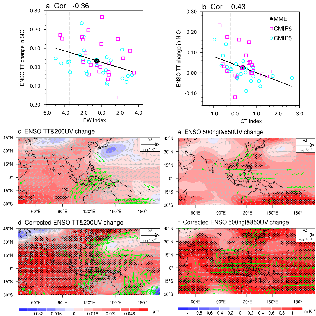
FIG. 8. (a) Scatterplots of the SON EW index vs projected changes in Niño-3.4-regressed tropospheric temperature anomalies over the south Indian Ocean during JJA(1). (b) Scatterplots of the DJF CT index vs projected changes in Niño-3.4-regressed tropospheric temperature over the northern Indian Ocean in 56 models. The intermodel correlation coefficients of the 56 models are shown in the top left of the panels. All correlation coefficients are significant at the 99% confidence level, based on the Student's t test. (c) MME changes in ENSO-related tropospheric temperature (925–200-hPa mean) and 200-hPa wind anomalies in the period 2070–96 relative to those in 1979–2005. (d) Observational constraint on changes in ENSO-related tropospheric temperature and 200-hPa wind anomalies. (e) MME changes in ENSO-related 500-hPa geopotential height and 850-hPa wind anomalies and (f) their observationally constrained counterparts.
