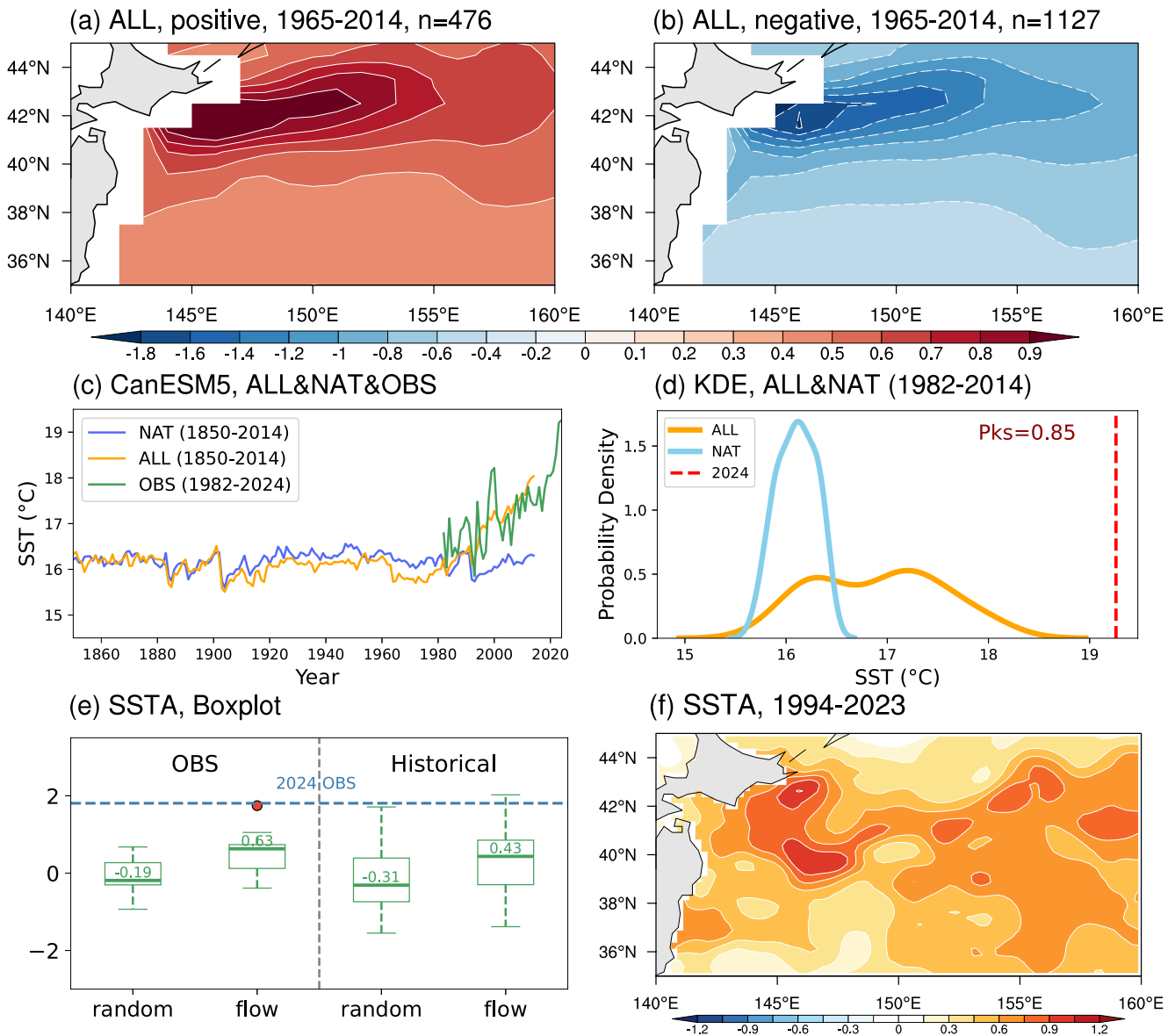
Figure 4. (a, b) Composite spatial patterns of KE SSTA associated with pronounced positive (a) and negative (b) SSTA in the NA. (c) Time series of the observed and simulated MJJAS sea surface temperature (SST) averaged over the KE region ( ^{\circ}\text{C} ). Orange and blue lines represent the ensemble means from CanESM5 historical simulations with all forcings (ALL) and natural forcings only (NAT) during 1850–2014, respectively. (d) Probability density functions (PDFs) of SST averaged over the KE region from CanESM5 simulations under ALL (orange) and NAT (blue) forcings. The vertical red dashed line indicates the observed SST in 2024. (e) Distributions of KE regional averaged SSTA ( ^{\circ}\text{C} ) for randomly selected years (first and third boxplots) and for years identified via the flow analog method (second and fourth boxplots), based on observations and CanESM5 historical simulations during 1994–2023. The boxplot shows the 25th percentile, median, and 75th percentile (bottom to top), while the horizontal blue dashed line marks the 2024 event threshold. (f) Composite spatial distribution of SSTA ( ^{\circ}\text{C} ) during the flow analog years in the observations, indicating typical patterns associated with similar atmospheric circulation to that in 2024.
