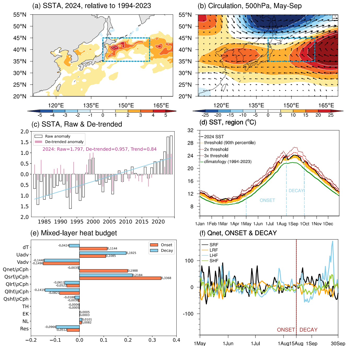
Figure 1. (a) Spatial distribution of SSTA (°C, shading) during MJJAS 2024. The blue box (35°–45°N, 140°–160°E) delineates the KE region analyzed in this study. (b) Anomalies of 500-hPa eddy geopotential height (gpm, shading) and winds (m/s, vectors) during MJJAS 2024. (c) Time series of KE-averaged SSTA (black bars), linear trend (blue line), and detrended anomalies (pink bars) during MJJAS from 1982 to 2024. (d) Daily sea surface temperature (SST) evolution in 2024 (°C, black), along with the climatological mean SST (°C, green), and the 90th percentile threshold of the 5-day running mean SST (°C, orange dashed line) used to define Category I (moderate) MHWs. Red and brown dashed lines indicate thresholds for Category II (strong) and Category III (severe) MHWs, respectively. The color shading beneath the SST curve denotes the MHW category for each day. The onset and decay phases of the 2024 MHW event are labeled in blue. (e) Bar chart of mixed-layer heat budget terms (°C/day) during the onset (orange) and decay (blue) phases of the 2024 KE MHW, including the temperature tendency ( dT ), zonal and meridional advection ( Uadv , Vadv ), Q_{net} , Q_{SRF} , Q_{LRF} , Q_{LHF} , Q_{SHF} , thermocline feedback (TH), upwelling feedback (EK), nonlinear (NL), and the residual term (Res). (f) Daily evolution of surface heat flux component anomalies ( W/m^2 ): Q_{SRF} (black), Q_{LRF} (orange), Q_{LHF} (blue), and Q_{SHF} (green) during MJJAS 2024.
