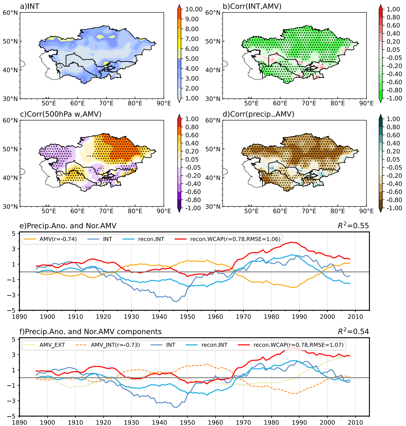
Figure 4. (a) One standard deviation for the internal component of the WCAP changes (unit: \text{mm month}^{-1} \text{decade}^{-1} ). (b) Correlation of internal component of WCAP anomalies and AMV index at each grid over CA. The dotted regions indicate significance at the 90% level. (c, d) Same as (b), but for 500-hPa vertical pressure velocity and precipitation, respectively. (e) Time series of AMV index (yellow line) and internally generated component of WCAP anomalies in the observation (dark blue). AMV-based reconstructed time series of internally generated component (light blue) and WCAP anomalies (red line). The numbers in the left legend and at upper right corner indicate the correlation coefficient and goodness-of-fit (square correlation) between AMV and internally generated component of observed WCAP anomalies, respectively. The number in the right legend indicates the correlation coefficient and RMSE of WCAP between in observation and reconstruction. (f) Same as (e), but AMV is further separated into externally forced (AMV_EXT) and internal (AMV_INT) components. The reconstruction of internally generated component (light blue) and WCAP anomalies (red line) is based on the AMV_INT. All variables are averaged at 11-year running window.
