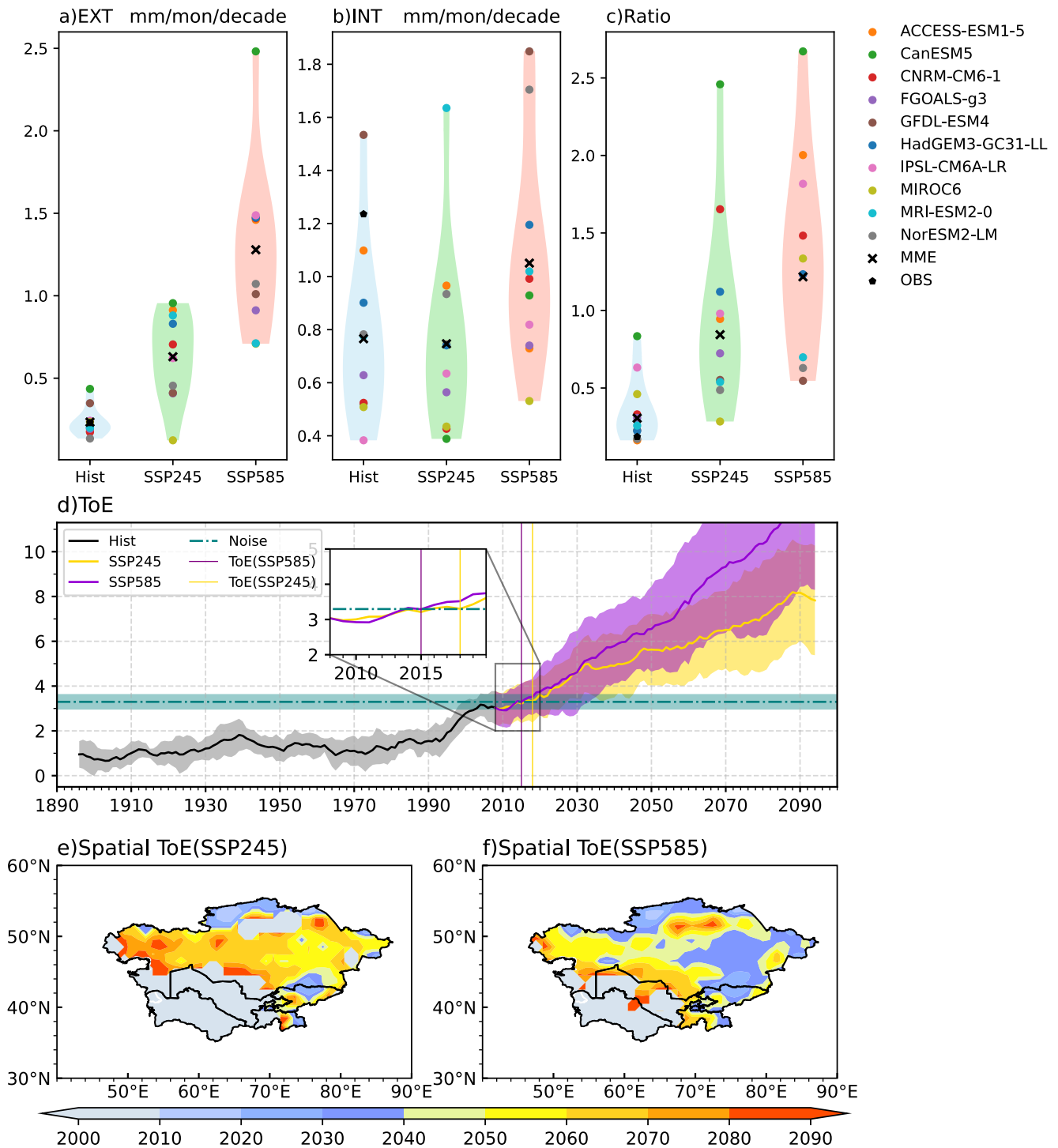
Figure 7. (a) The violin and scatter plot of 21-year running externally forced WCAP trends (unit: \text{mm month}^{-1} \text{ decade}^{-1} ) for each model, MME and observation in historical simulations (1891–2014), SSP2–4.5 (2015–2099), and SSP5–8.5 (2015–2099) scenarios. (b, c) Same as (a), but for one standard deviation (unit: \text{mm month}^{-1} \text{ decade}^{-1} ) and the ratio between panels (a) and (b). (d) The 11-year running averaged time series of externally forced WCAP anomalies (unit: \text{mm} ) in historical simulations (black), SSP2–4.5 (yellow) and SSP5–8.5 (purple) scenarios. The shadings indicate the corresponding one standard deviation among models. The inset figure is to clarify the ToE. The yellow and purple vertical lines for SSP2–4.5 and SSP5–8.5 scenarios indicate year of 2018 and 2015, respectively. (e) The spatial distribution of ToE under SSP2–4.5 scenario at each grid over CA. (f) Same as (e), but under SSP5–8.5 scenario.
