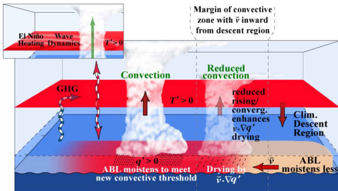
Fig. 3 Schematic diagram of the upped-ante mechanism and the anomalous gross moist stability (rich-get-richer) mechanism. Adapted from Neelin and Su (2005) .
