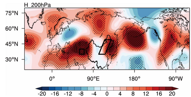
Fig. 10 The regression patterns of the geopotential height (contour, unit: gpm) at 200 hPa in summer (JJA) during 1979–2010 onto standardized interannual component of CGTI, respectively. Dots indicate significant at the 95% confidence level
