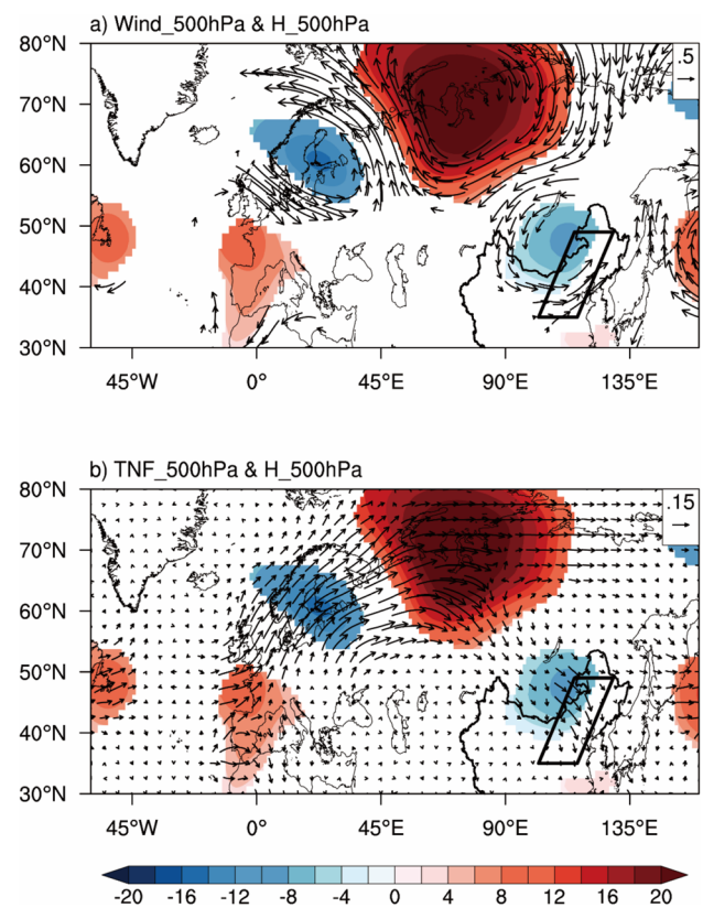
Fig. 4 a The regression map of horizontal wind (a, vector, unit: \text{m s}^{-1} ) and geopotential height (shading, unit: gpm) at 500 hPa in summer (JJA) during 1979–2010 onto standardized interannual component of EUI, as well as the corresponding horizontal wave activity flux (b, vector units: \text{m}^2\text{s}^{-1} ). Horizontal wind and the geopotential height are significant at the 95% confidence level
